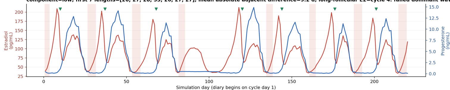
C. Healthy age 52, later-life long-cycle episode component=low; first 7 lengths=[26, 27, 28, 53, 26, 27, 27]; mean absolute adjacent difference=9.2 d; long-follicular E2=cycle 4: failed dominant wave
